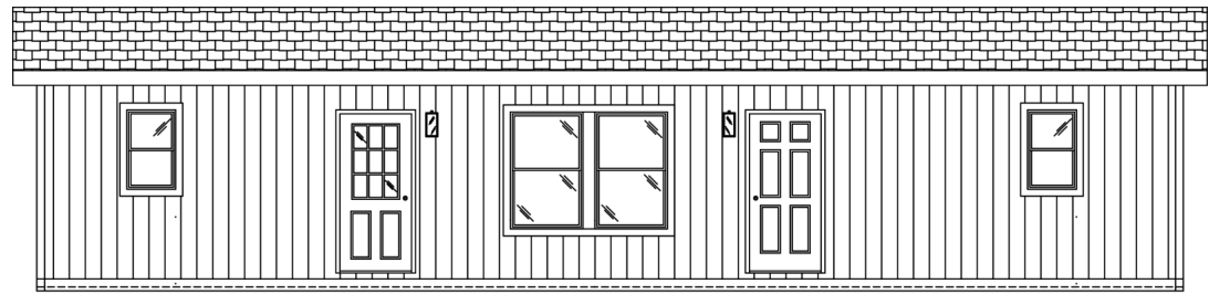
FRONT SIDEWALL
